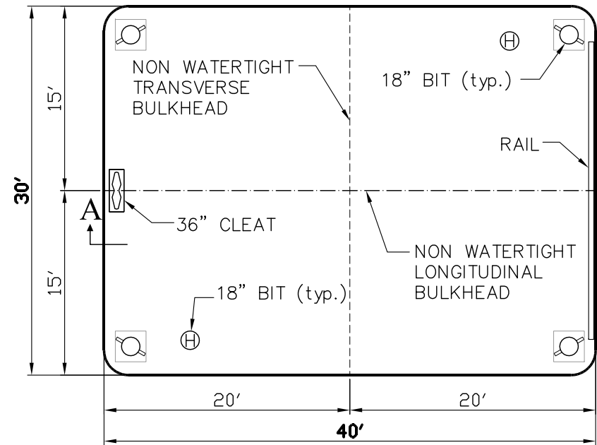
DECK PLAN
