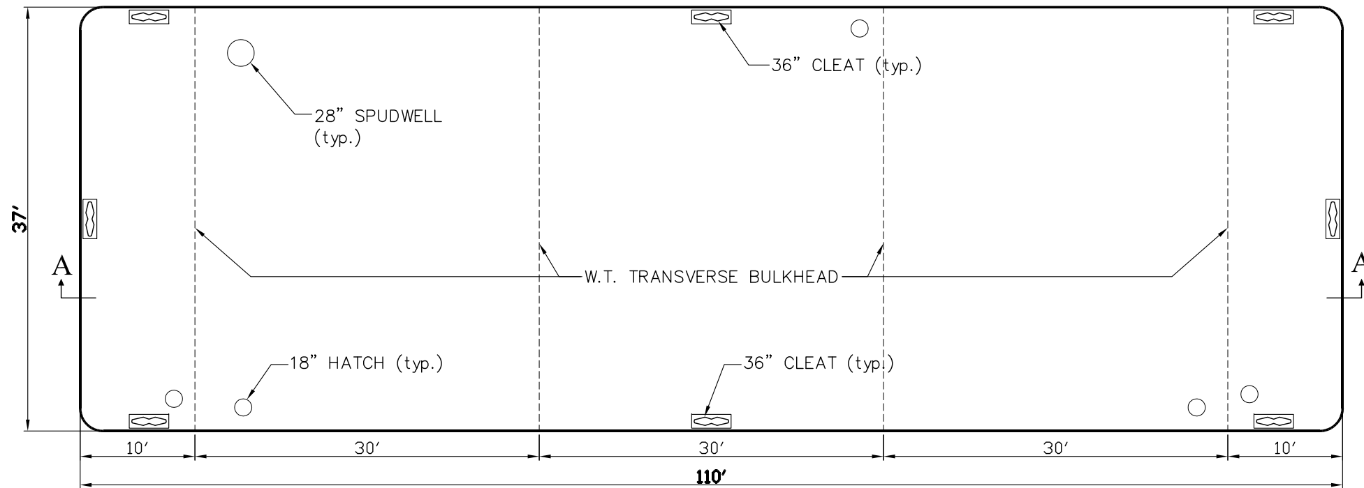
DECK PLAN
