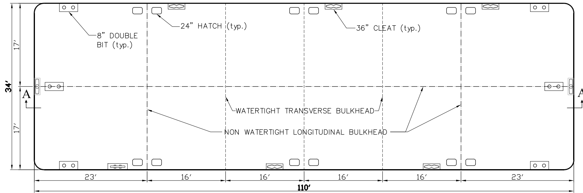
DECK PLAN
