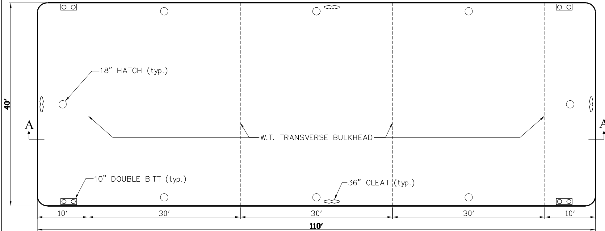
DECK PLAN
