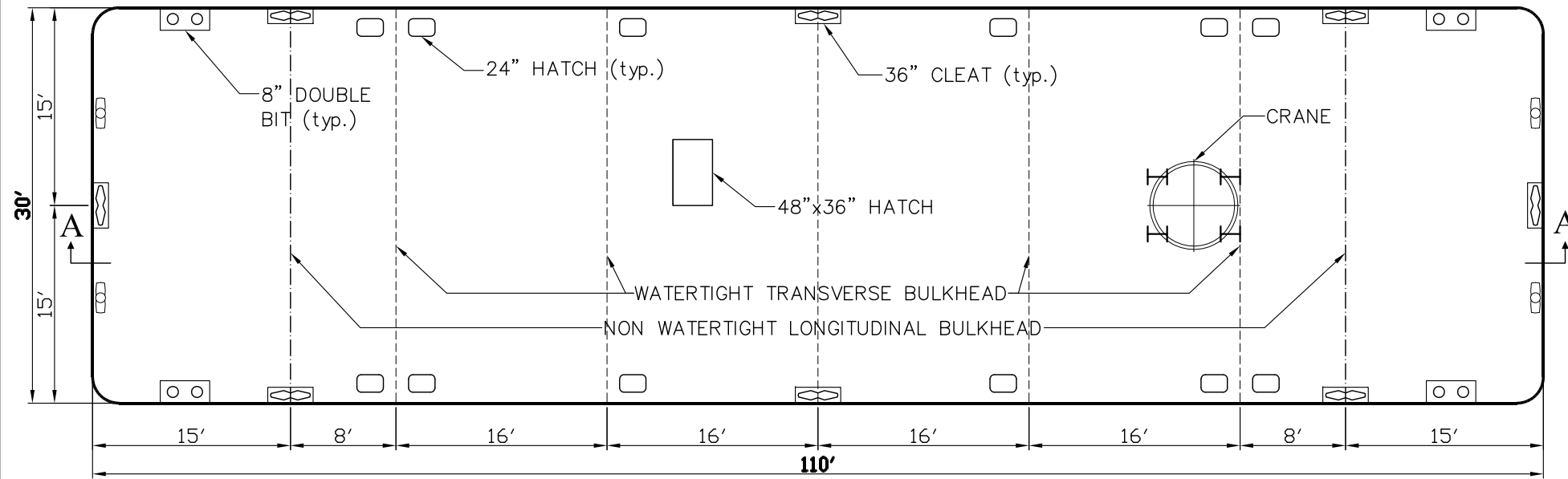
DECK PLAN
