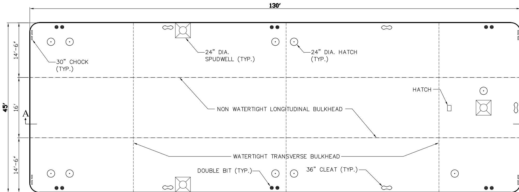
DECK PLAN
