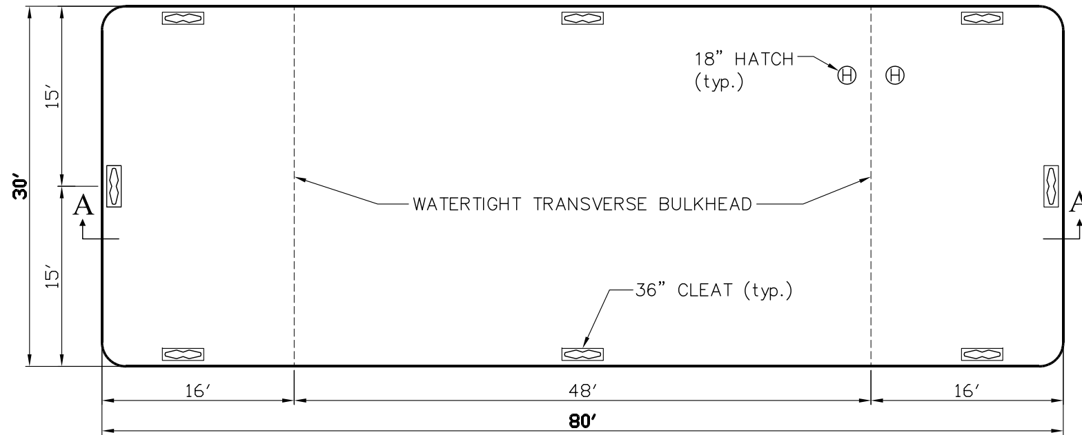
DECK PLAN
